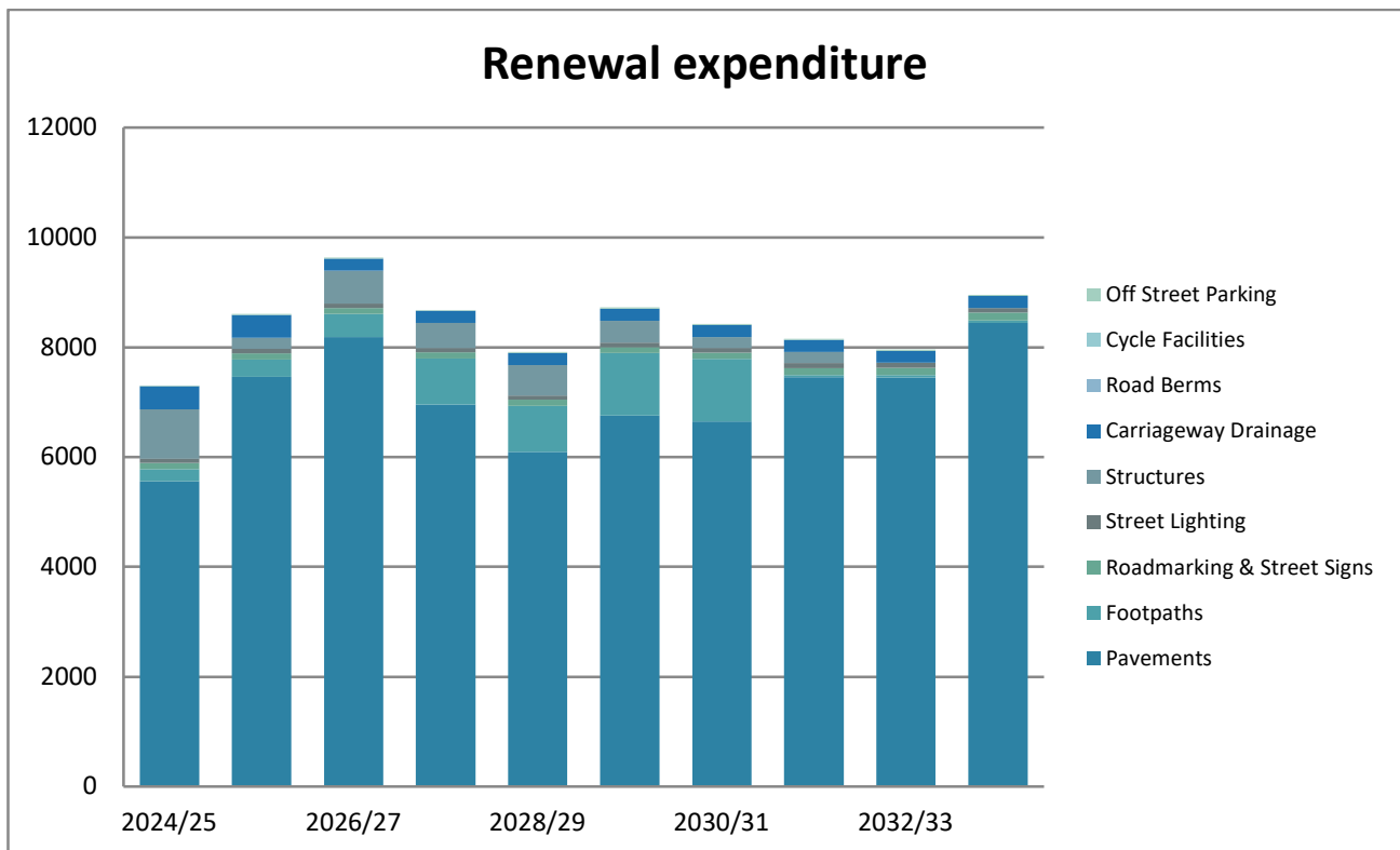
Figure 23. Renewal expenditure
