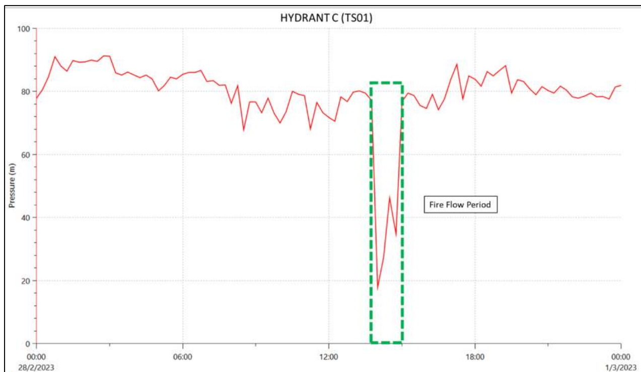
Residual pressure at Critical Hydrant C
