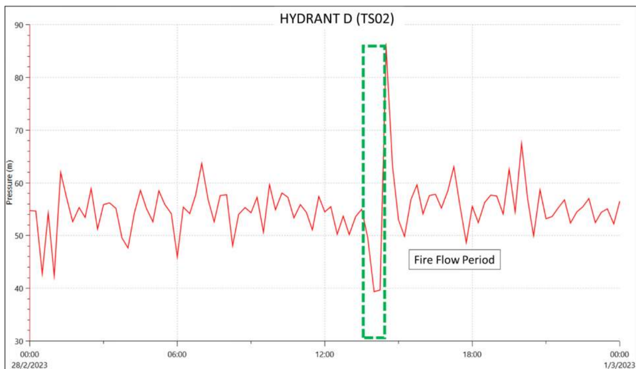
Residual pressure at Critical Hydrant D
