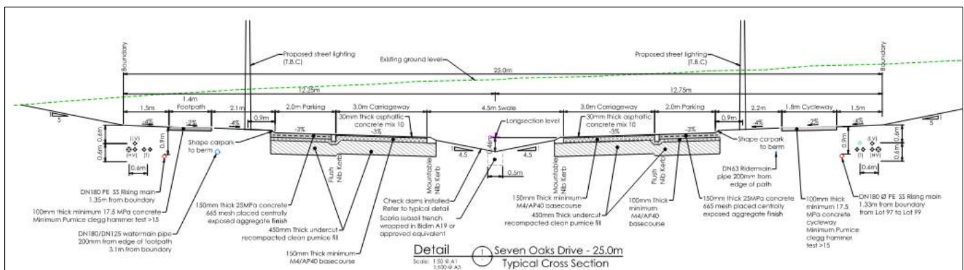
Figure 14 – Kahikatea Drive Typical Cross Section
