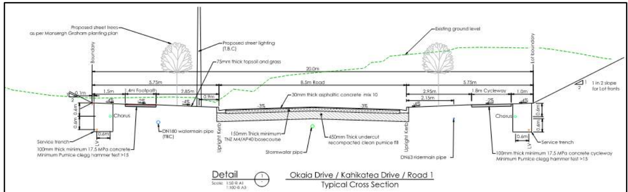
Figure 13 - Okaia Drive and Road 1 Typical Cross Section
