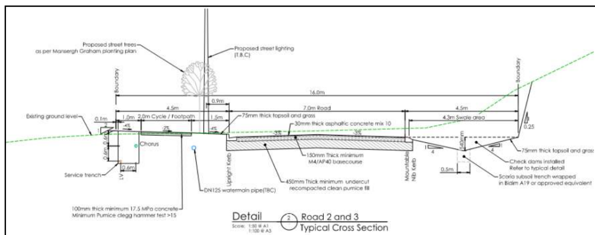
Figure 15 - Preliminary Cul-de-Sac Typical Cross Section
