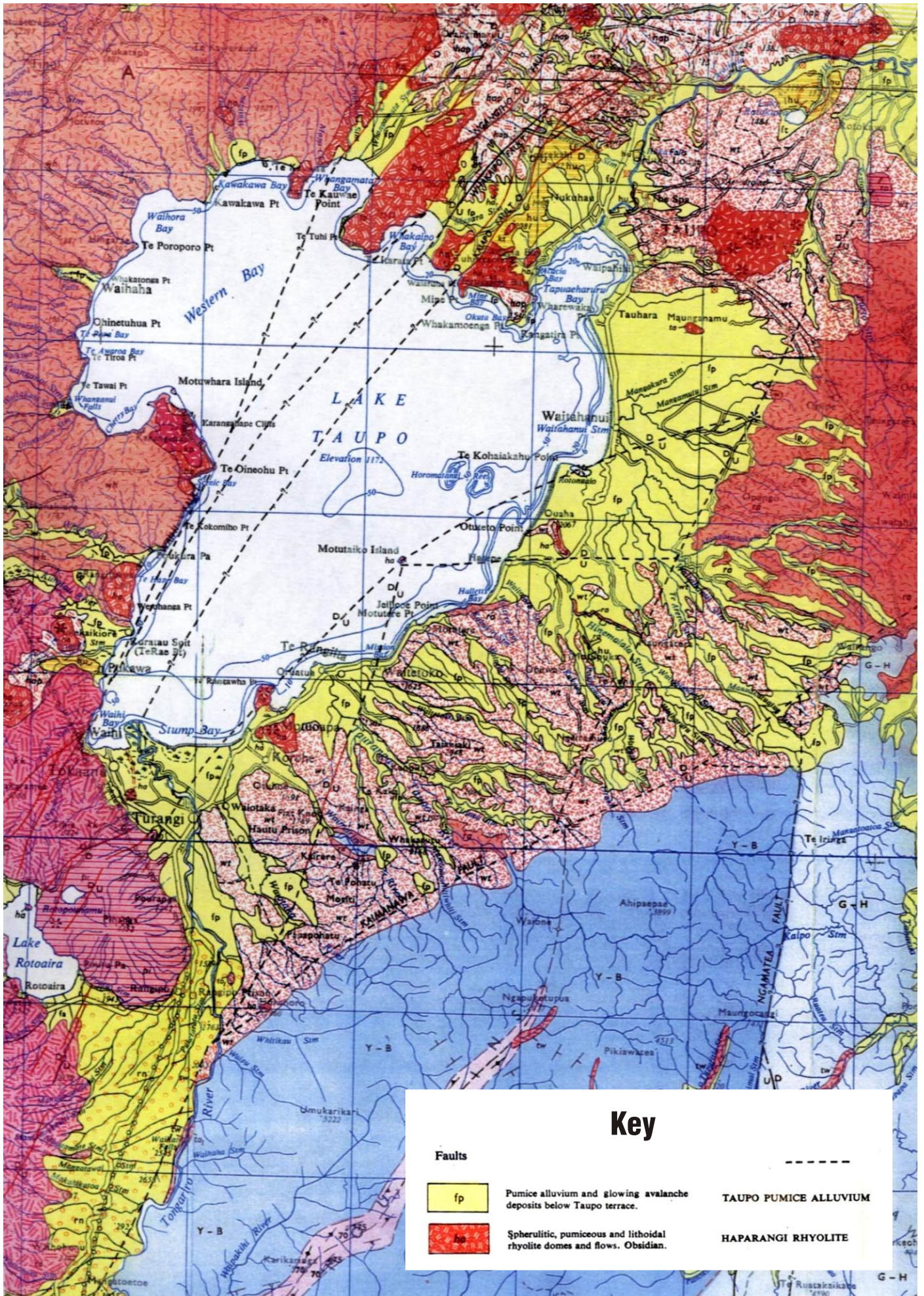
Geology of Area
